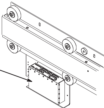
2206437 M4 X 12mm NYLON SCREW FOR SPEAKER GRILL
